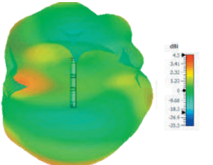
3D Plot Element D Top (2600 MHz)
